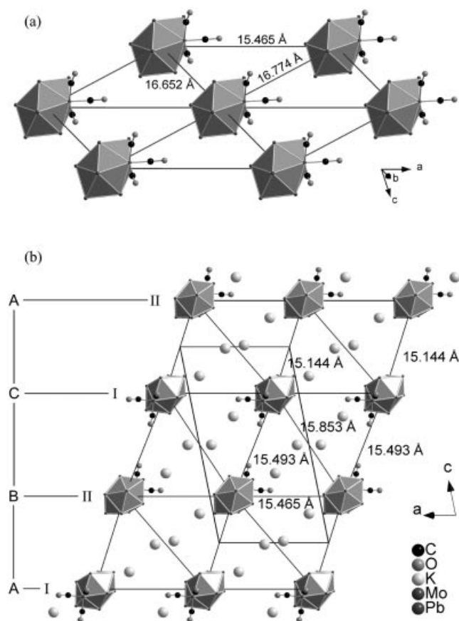
Figure 4. (a) The hexagonal packing in the ab plane in the single crystal of compound 1 . (b) The stacking sequence of the layers along the c axis in compound 1 (2.2.2-crypt units are not shown).
