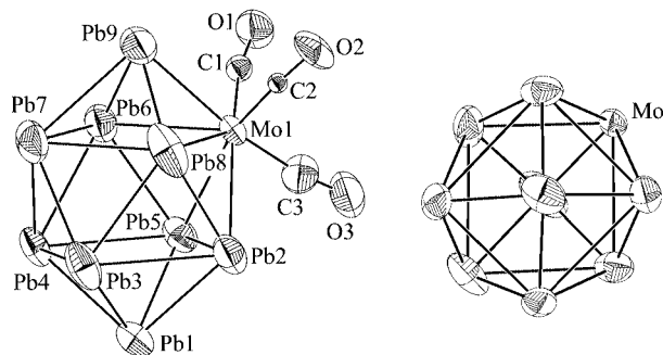
Figure 1. Molecular structure of the closo - [(\eta^5\text{-Pb}_9)\text{Mo}(\text{CO})_3]^{4-} unit in compound 1 (thermal ellipsoids set at 80% probability).
