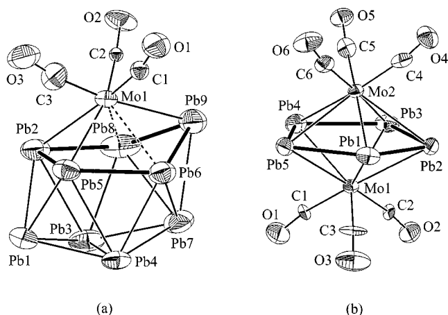
Figure 3. (a) Molecular structure of the closo -[( \eta^5 -Pb 9 )Mo(CO) 3 ] 4- unit in compound 1 (thermal ellipsoids set at 80% probability) (dotted lines represent Mo–Pb distances > 3.2 Å). (b) The structure of the closo -[ \eta^5 -Pb 5 {Mo(CO) 3 } 2 ] 4- Zintl anion (thermal ellipsoids set at 80% probability).
