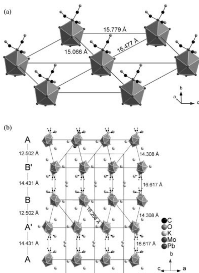
Figure 5. (a) The hexagonal packing in the ac plane in the single crystal of compound 2 . (b) The stacking sequence of the layers along the b axis in compound 2 (2.2.2-crypt units are not shown).
