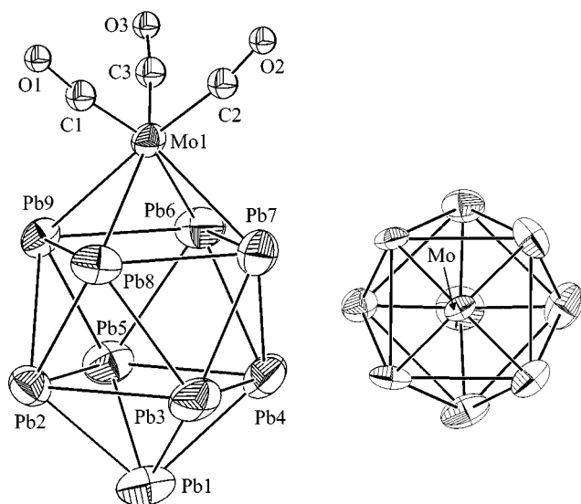
Figure 2. Molecular structure of the closo -[( \eta^4 -Pb 9 )Mo(CO) 3 ] 4- unit in compound 2 (thermal ellipsoids set at 50% probability).
